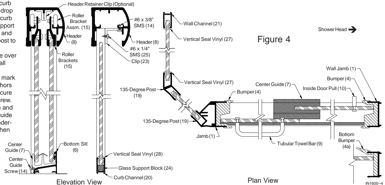
Elevation View
